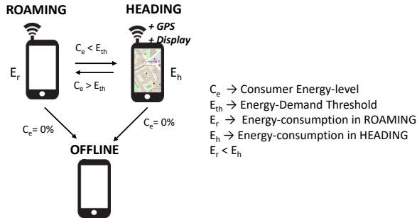
Figure 3. Mobile nodes resource consumption states.
