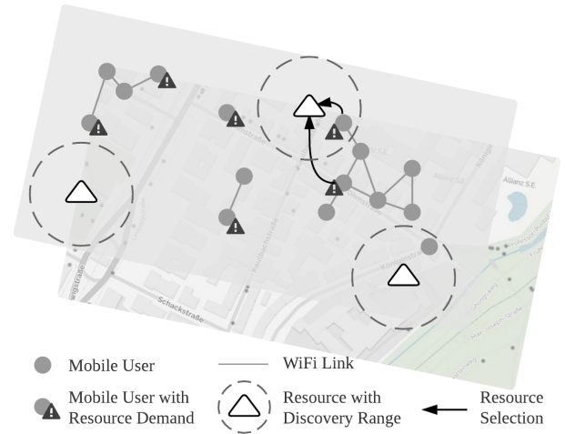
Figure 1. Entities in a post-disaster urban ad-hoc communication network. Physical resources can be discovered and consumed by mobile nodes that communicate via Wi-Fi. Adapted from [1].
